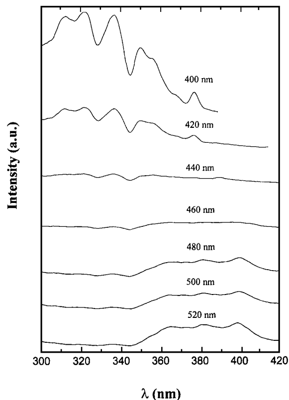
Fig. 5. Excitation spectra of a low-concentration PSC cyclohexane solution with an excess of propylamine at different emission wavelengths.
